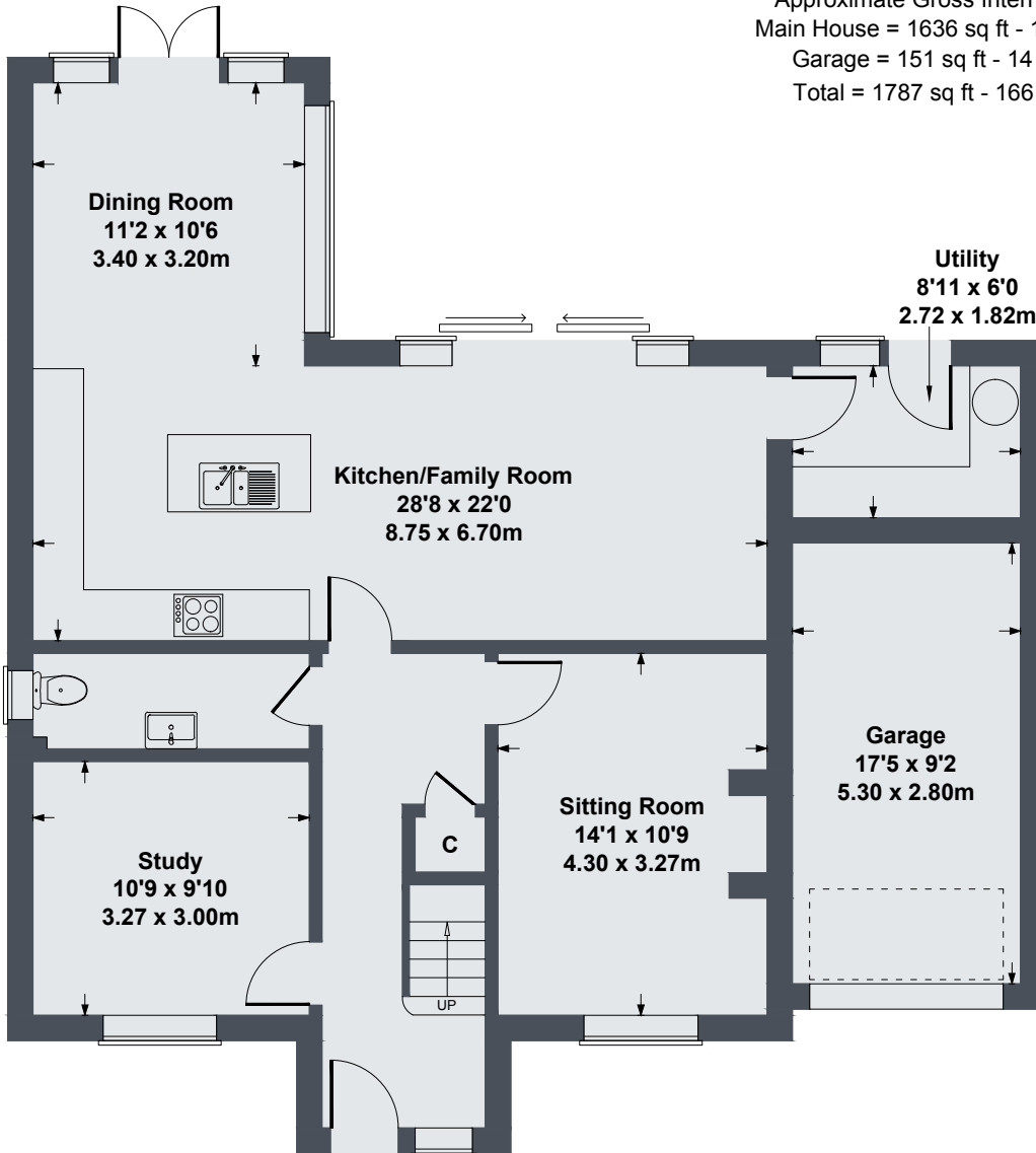
GROUND FLOOR
