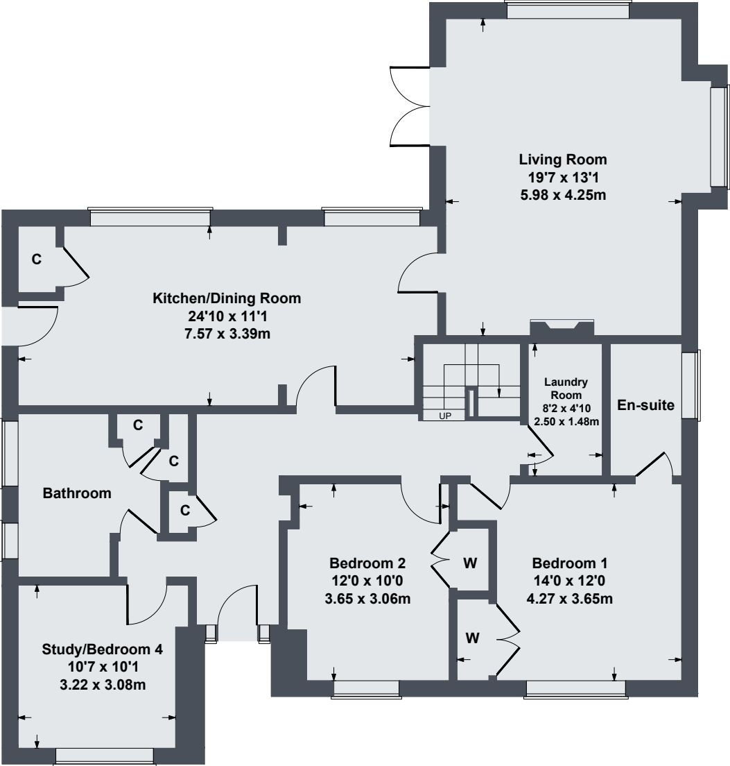
GROUND FLOOR
